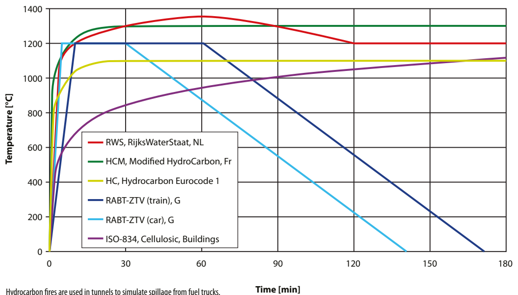
International Time/Temperature Curves used to test the fire-resistance ratings of passive fire protection systems in tunnels and buildings.
